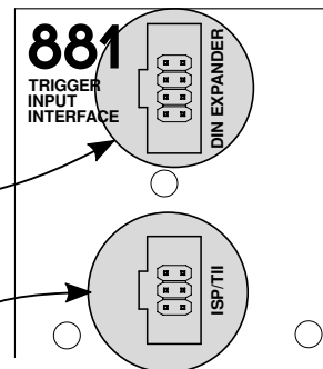
881 REAR PANEL
