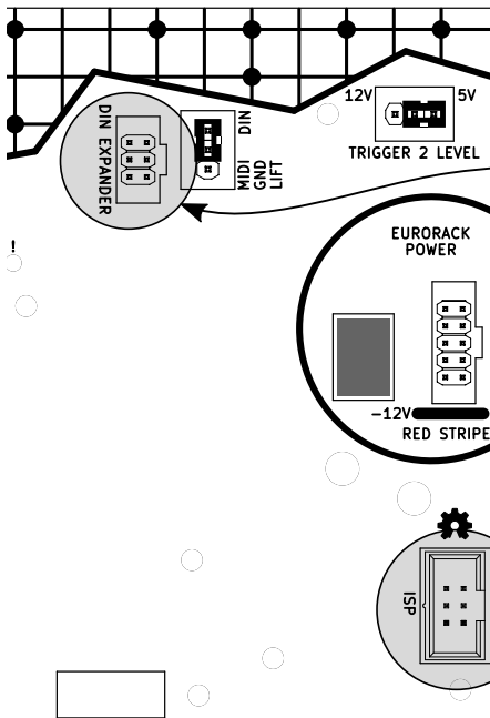
880 REAR PANEL
